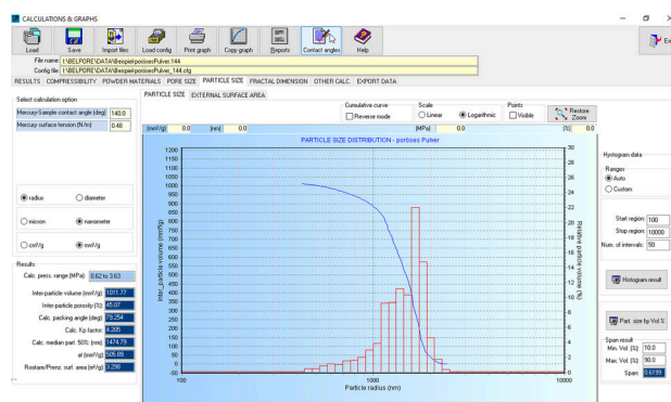
Evaluating Particle size with the PoreInspect software
