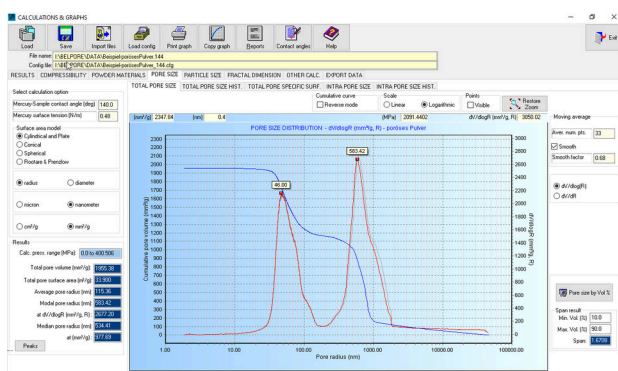
Evaluating pore size with the PoreInspect Software
